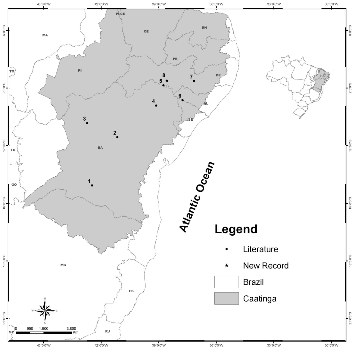
Figure 2. Records of Tropidurus cocorobensis . Bahia (BA): 1. Caeté (Freitas and Silva, 2007), 2. Morro do Chapéu (Freitas and Silva, 2007), 3. Xique-Xique (Freitas and Silva, 2007), 4. Canudos (Type-Locality, Rodrigues, 1987), 5. Rodelas (Rodrigues, 2003); Alagoas (AL): 6. Xingó (Rodrigues, 2003); Pernambuco (PE): 7. Buíque (Parque Nacional do Catimbau, Rodrigues, 2003; Muniz and Santos, 2009), 8. Floresta (new record).
